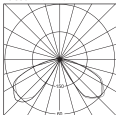
Facet L104 28W LED
